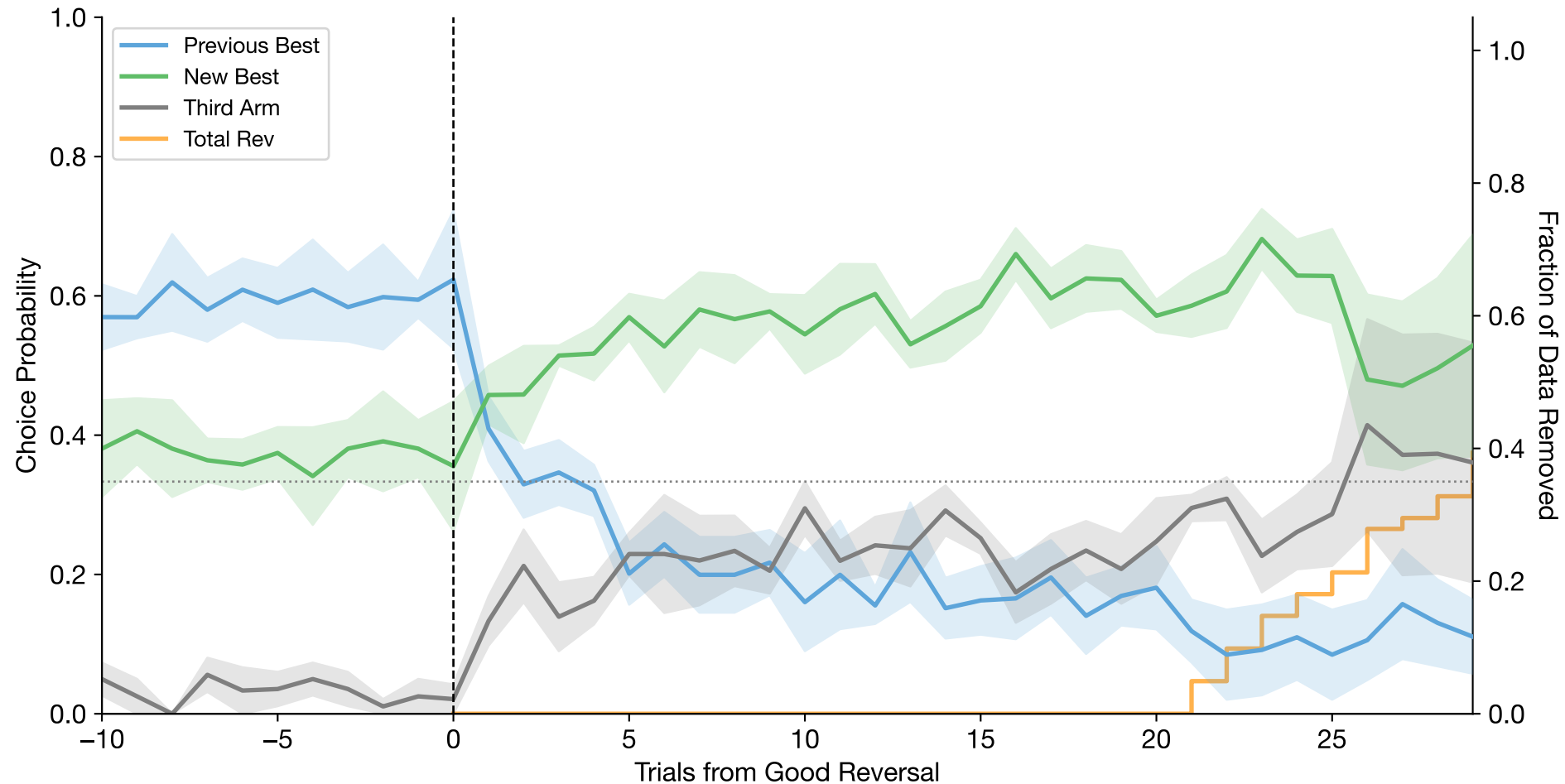
Good Reversal-Aligned Choices (mean \pm se across subjects | n=5 subjects, n=61 reversals)
